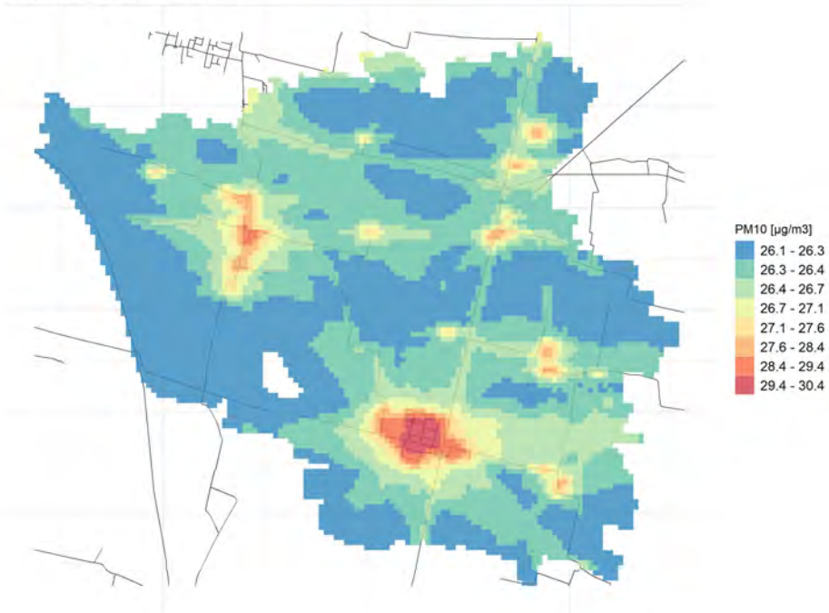
Conc. media annua PM10
