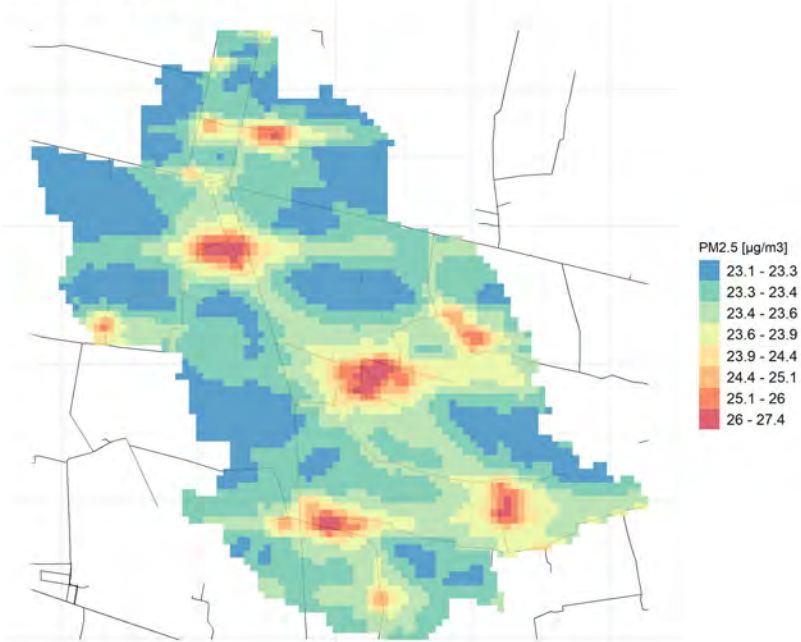
Conc. media annua PM2.5
