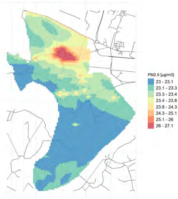
Conc. media annua PM2.5
