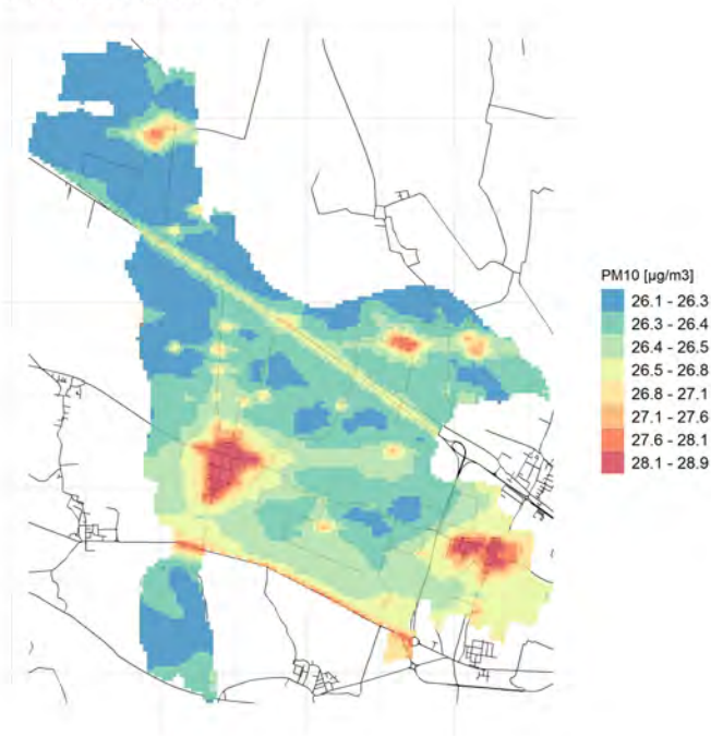
Conc. media annua PM10
