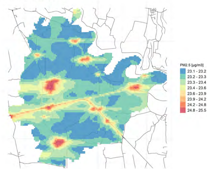
Conc. media annua PM2.5
