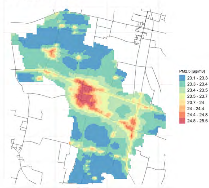
Conc. media annua PM2.5
