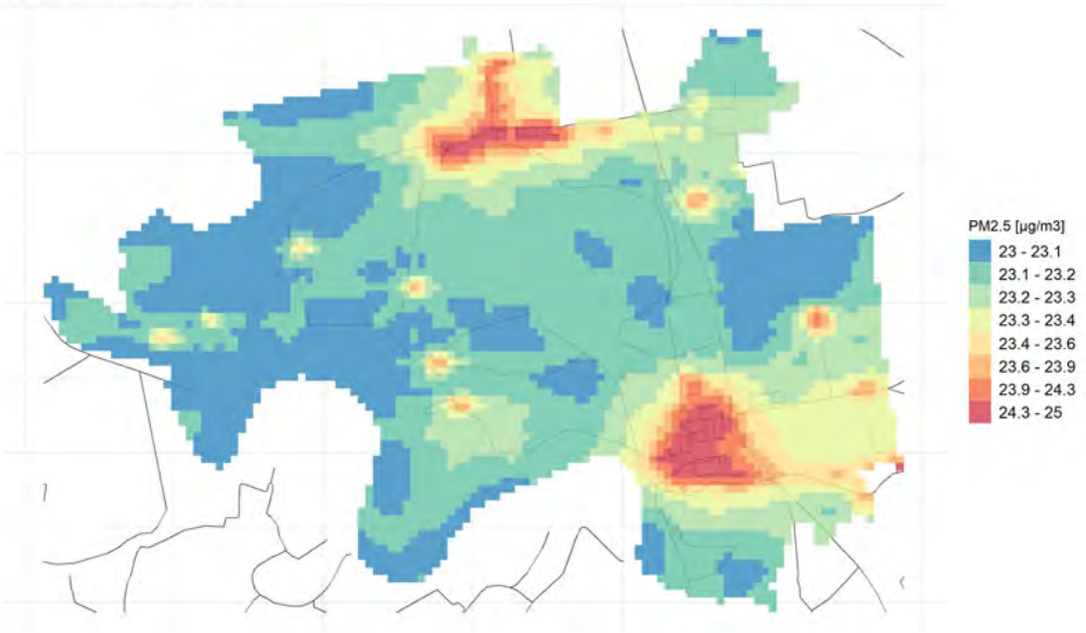
Conc. media annua PM2.5
