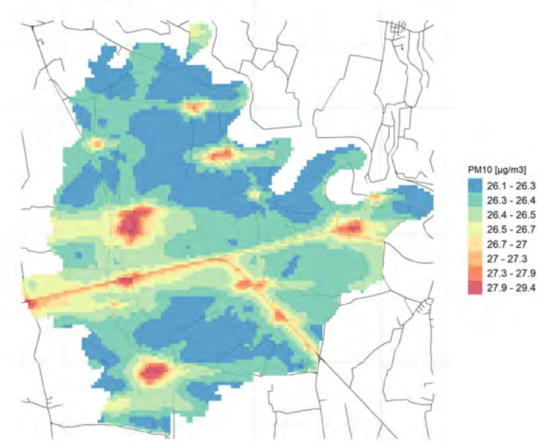
Conc. media annua PM10
