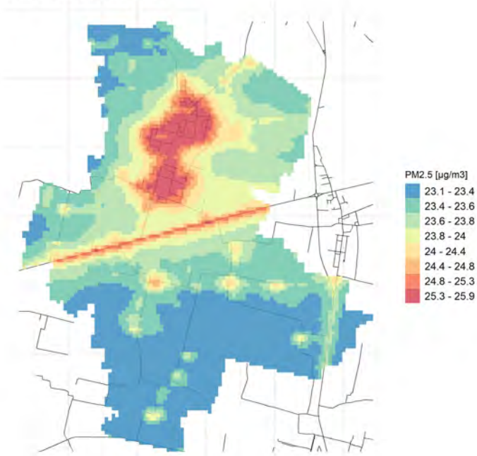
Conc. media annua PM2.5
