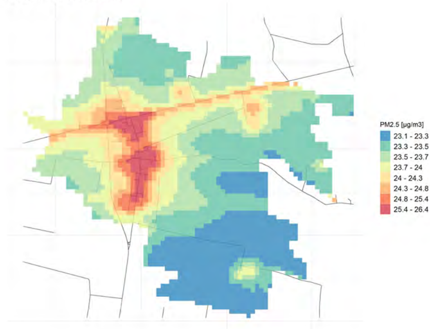
Conc. media annua PM2.5
