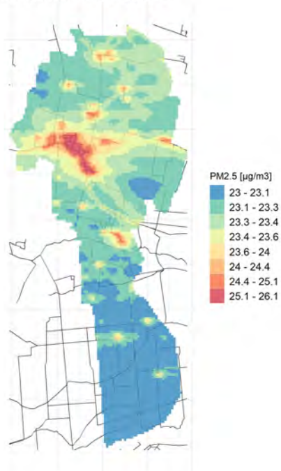
Conc. media annua PM2.5
