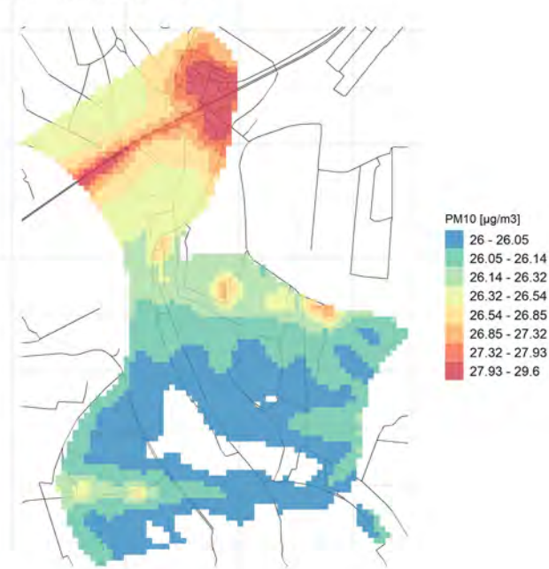
Conc. media annua PM10
