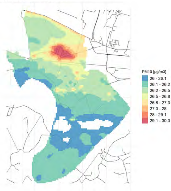
Conc. media annua PM10
