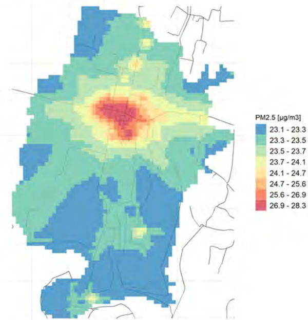
Conc. media annua PM2.5
