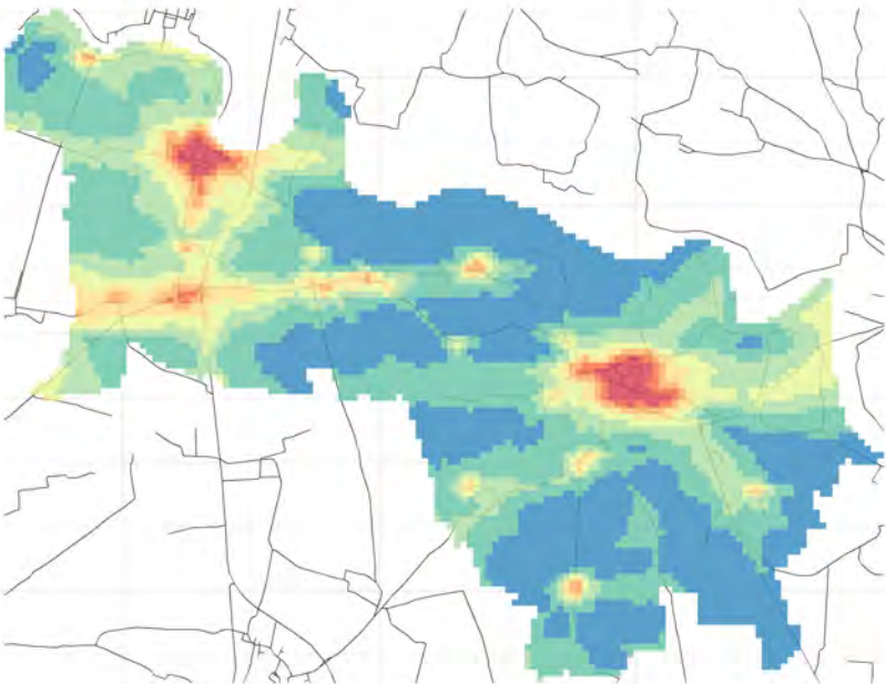
Conc. media annua PM10
