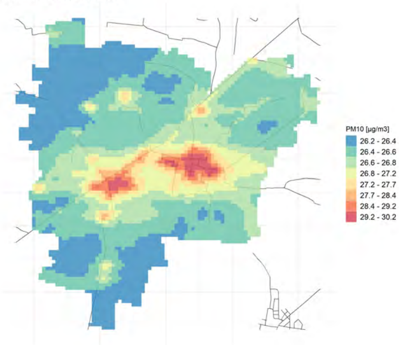
Conc. media annua PM10
