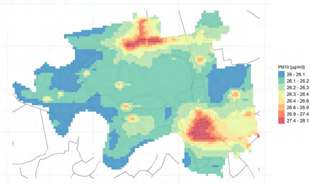
Conc. media annua PM10
