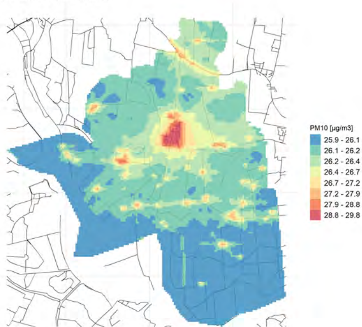
Conc. media annua PM10
