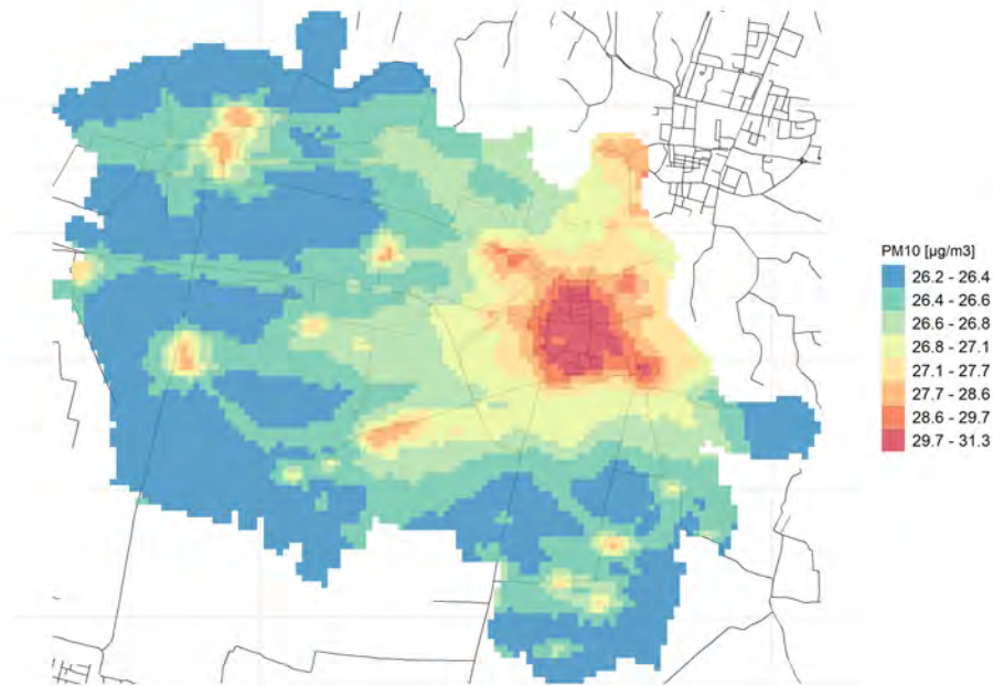
Conc. media annua PM10
