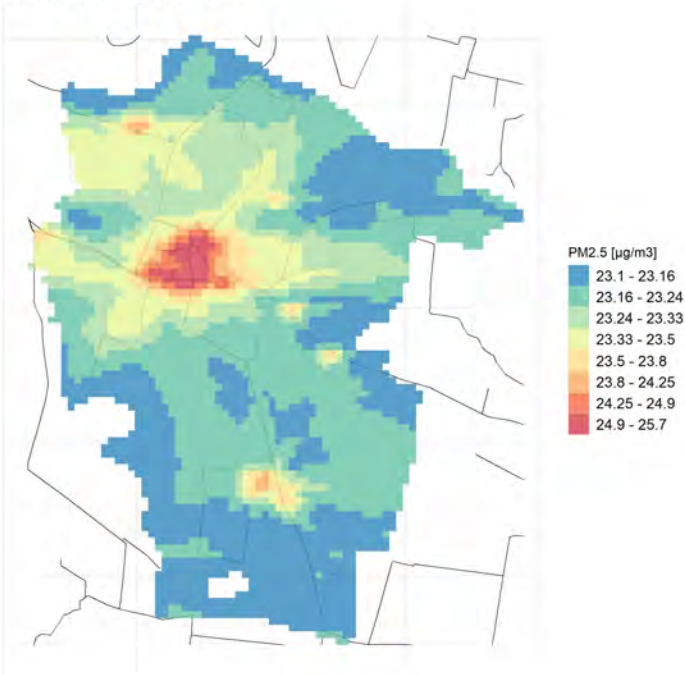
Conc. media annua PM2.5
