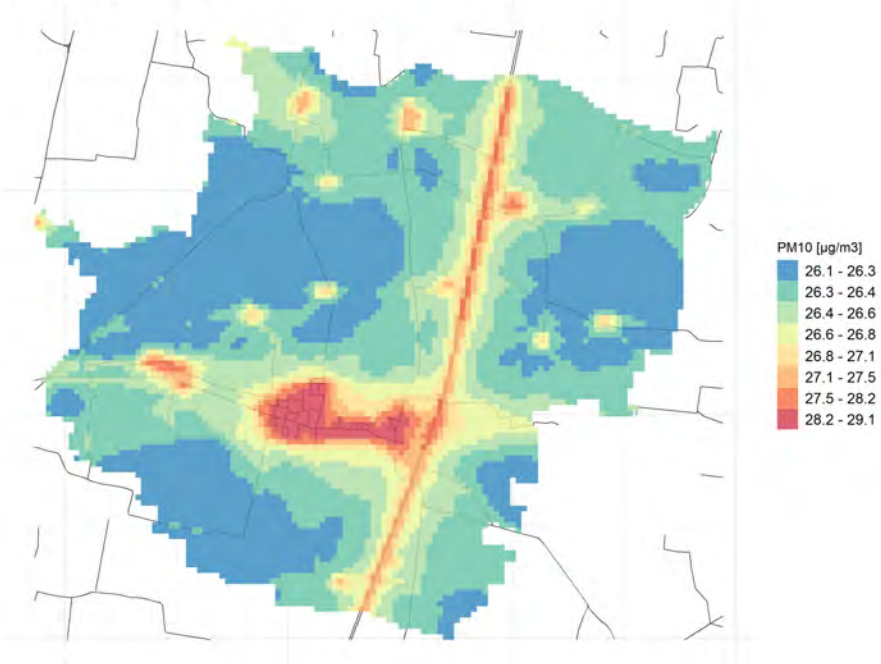
Conc. media annua PM10
