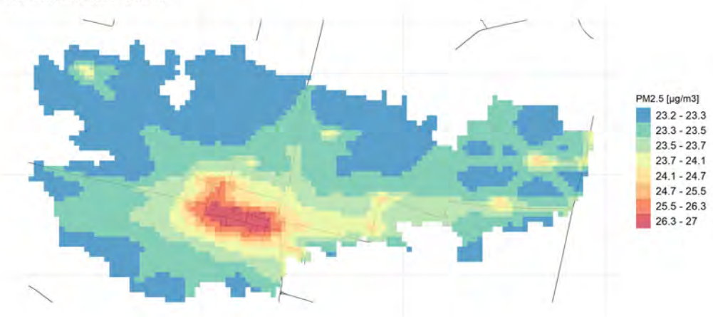
Conc. media annua PM2.5
