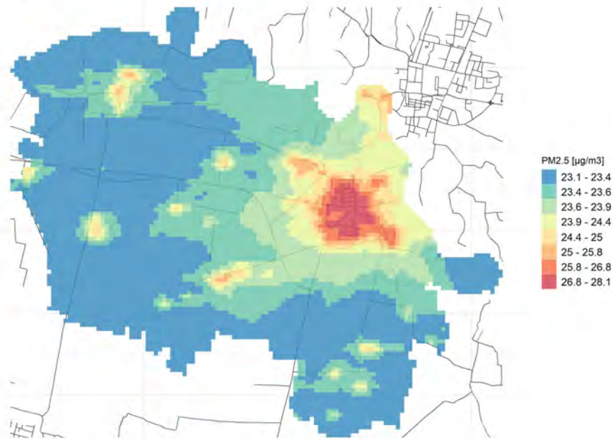
Conc. media annua PM2.5
