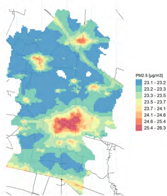
Conc. media annua PM2.5
