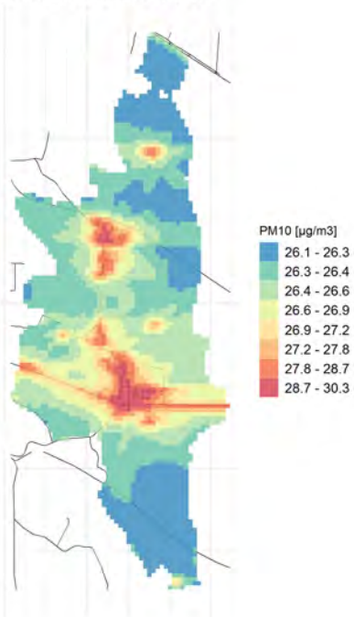
Conc. media annua PM10
