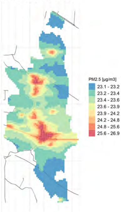
Conc. media annua PM2.5
