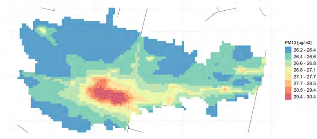
Conc. media annua PM10
